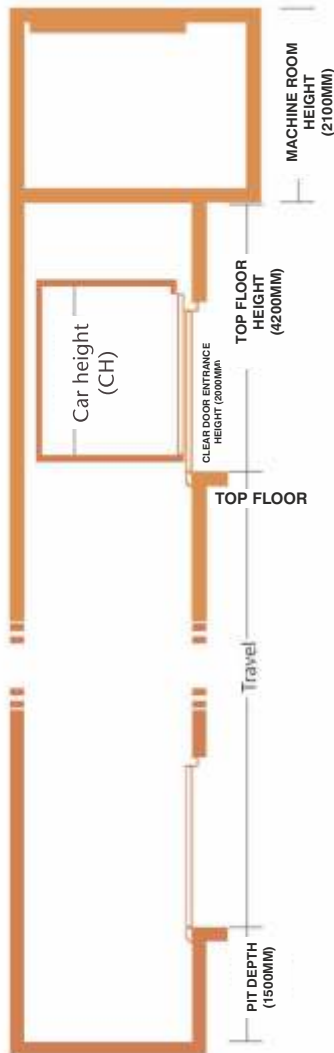
Lift with Machine Room (LMR)
